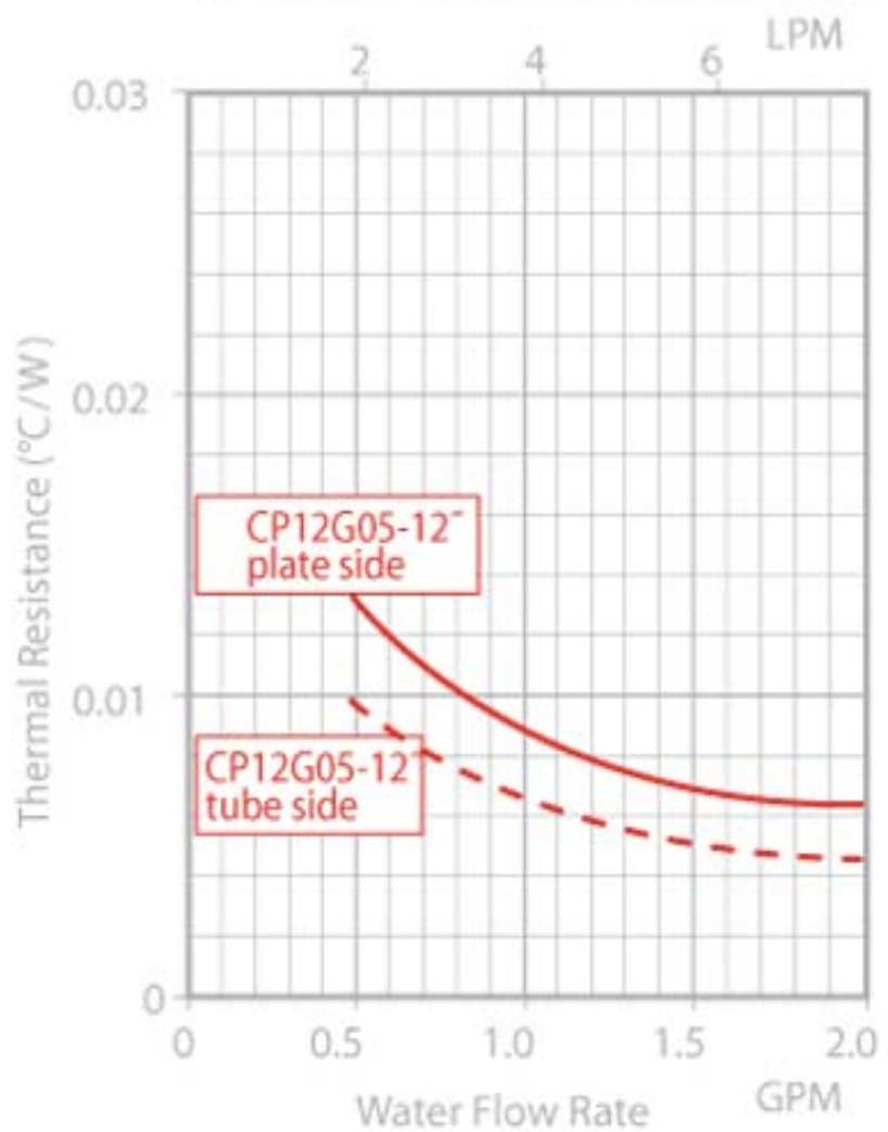
CP12G05 Thermal Resistance
