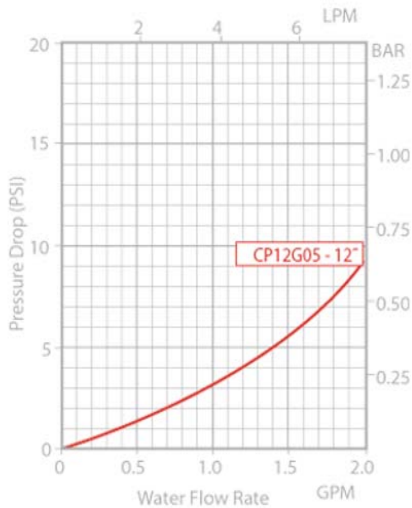
CP12G05 Pressure Drop
