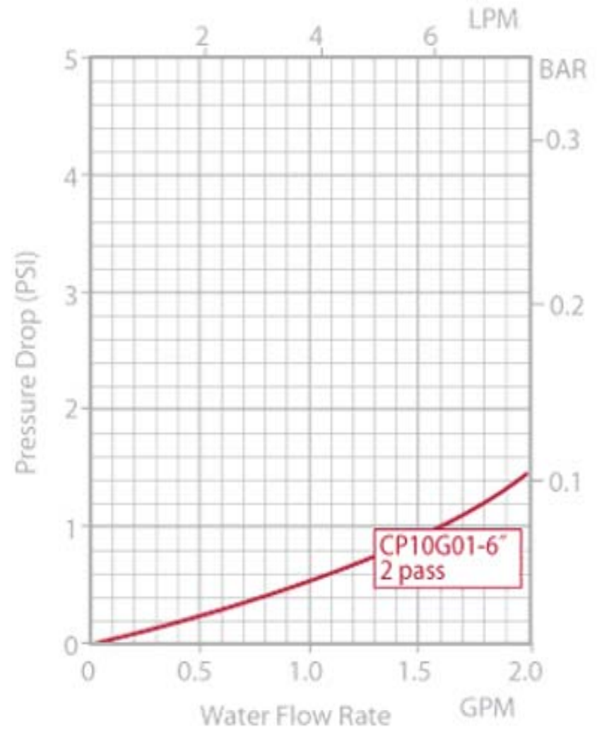
CP10G01 Pressure Drop
