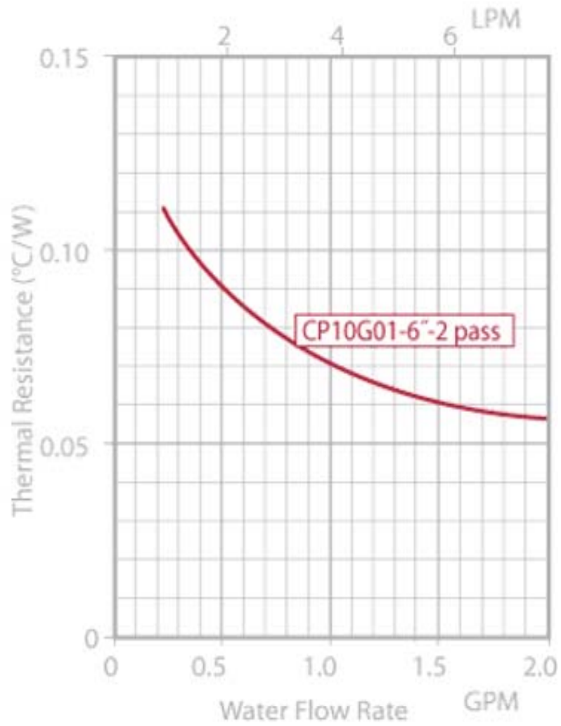
CP10G01 Thermal Resistance
